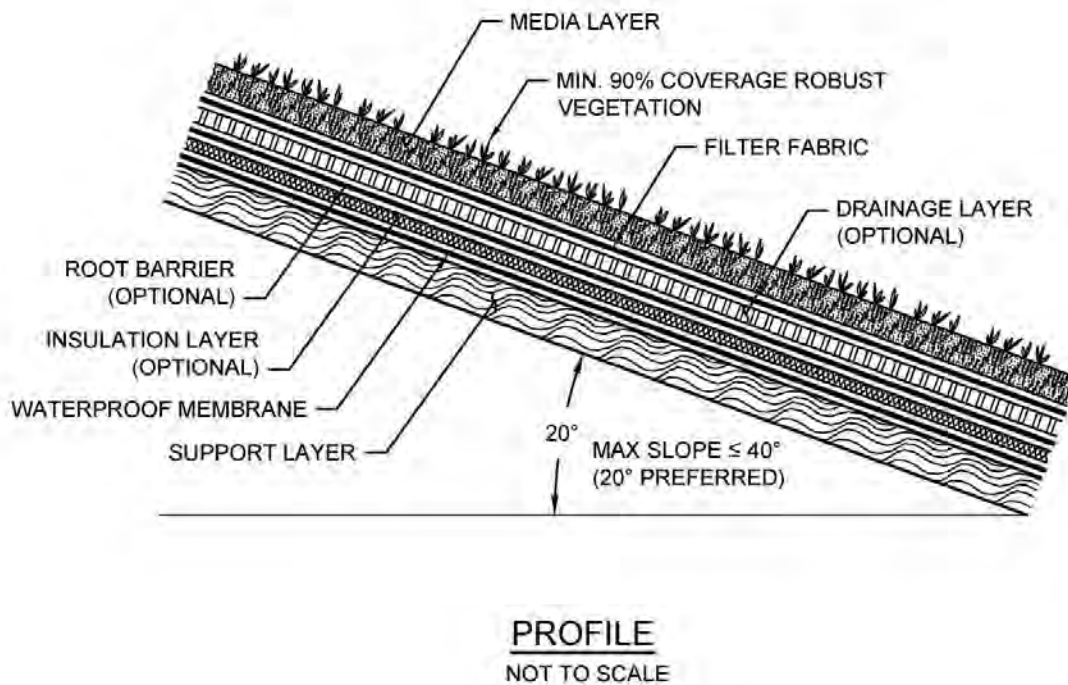
Typical Profile of a Green Roof BMP
