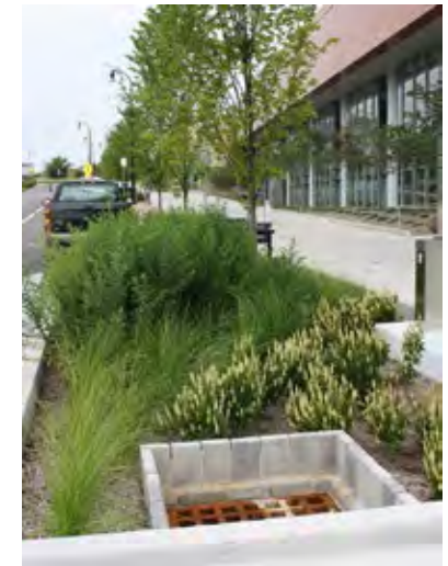
Figure 4-20. Concrete band structure constructed around the outflow allows ponding in Nashville, TN.
