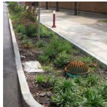
The overflow drain is placed in the flow path of water entering the practice.
