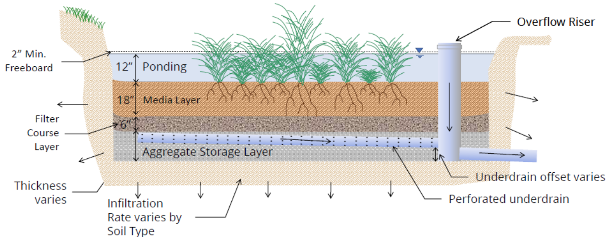
Biofiltration with Partial Retention BMP Example Illustration
