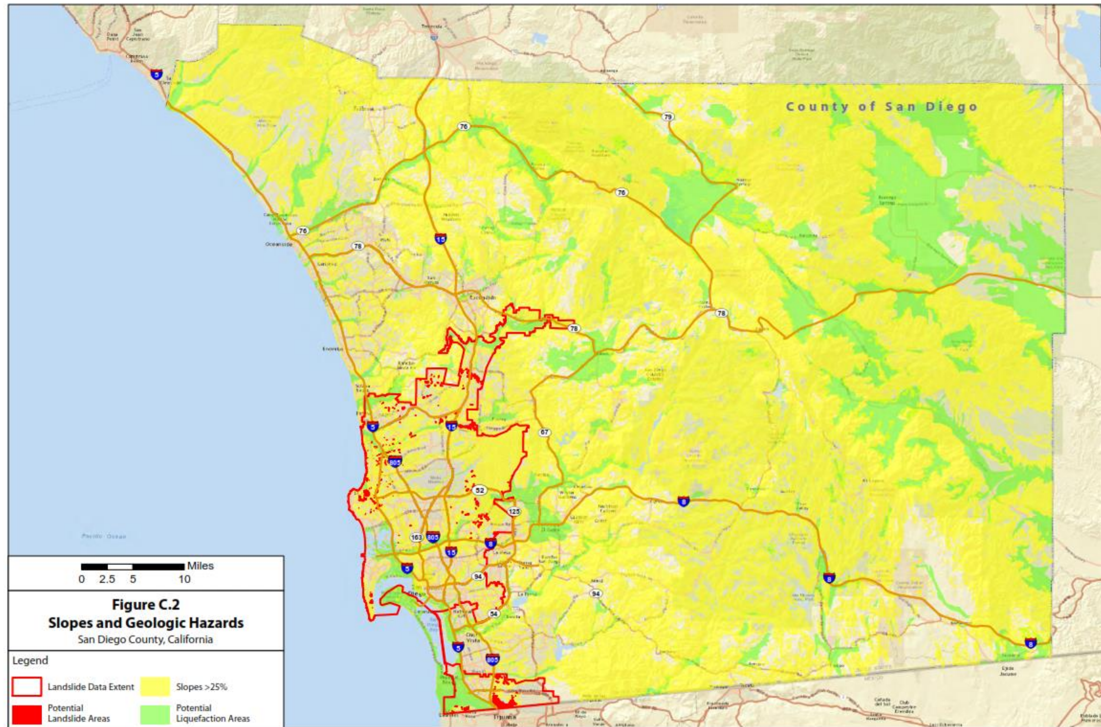
Figure C.2. Slopes and Geologic Hazards
