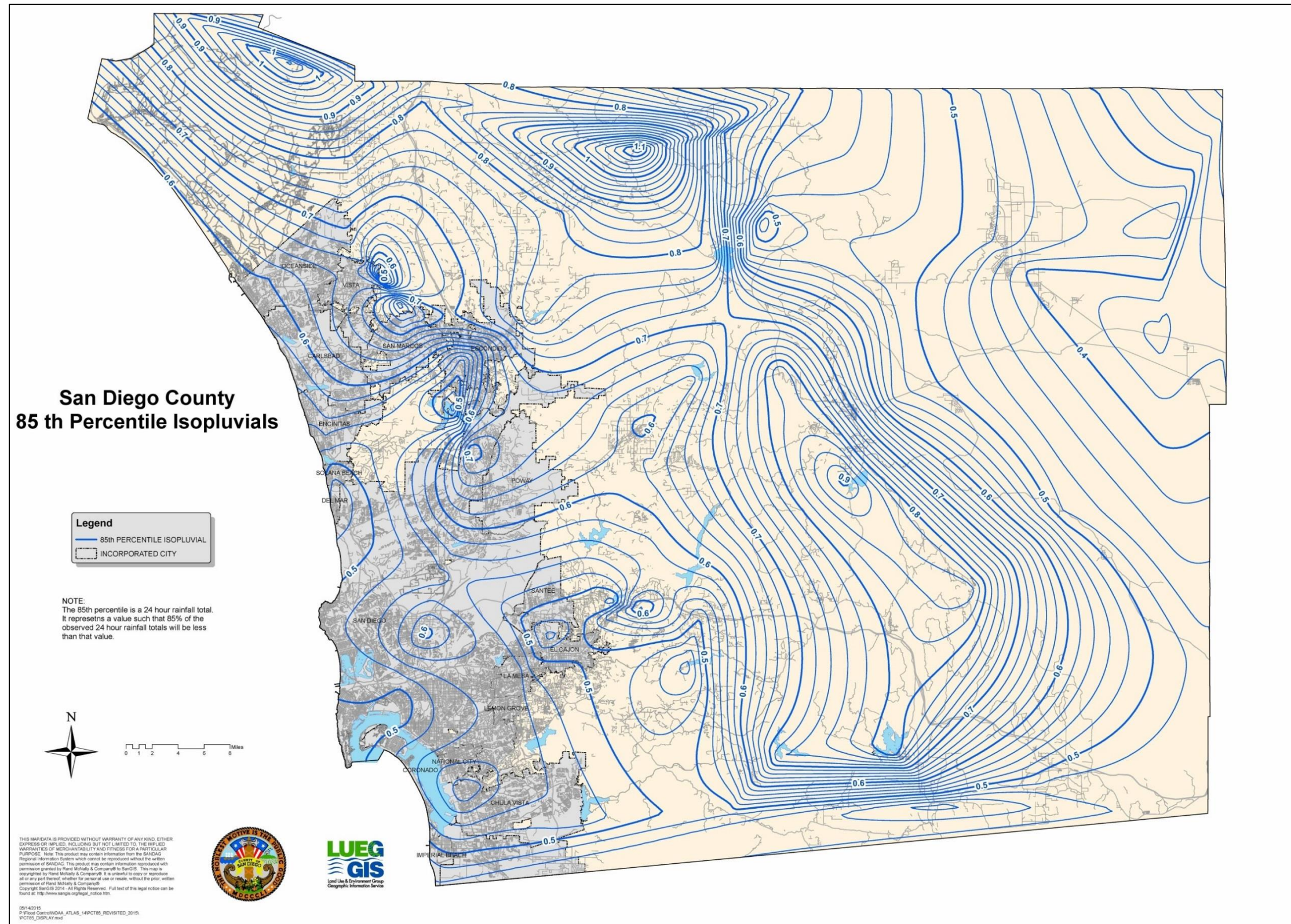
Figure B.1-1. 24-Hour, 85th Percentile Isopluvial Map
