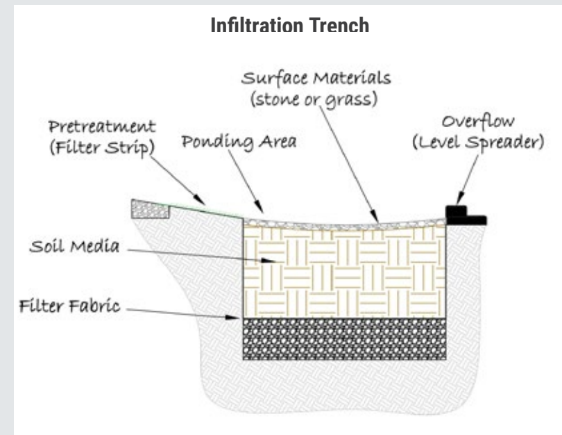
Figure 6-8. Stormwater infiltration trench schematic.
