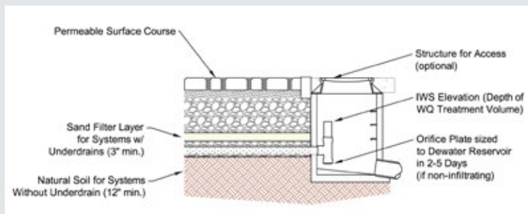
Figure 6-11. Permeable interlocking concrete pavement cross-section.
