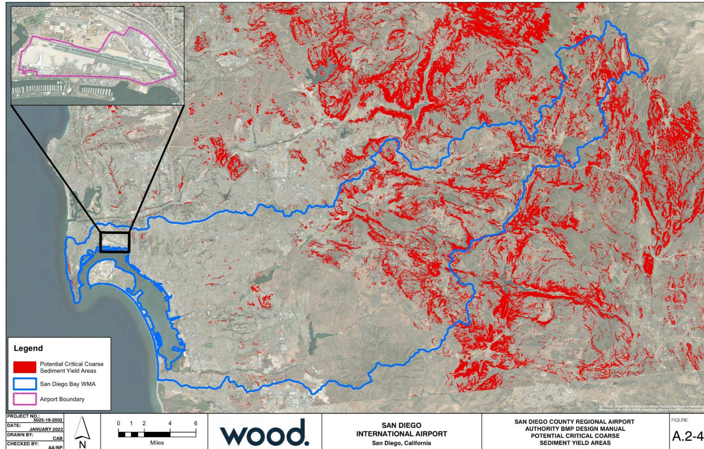
Figure A.2-4: Potential Critical Coarse Sediment Yield Areas
