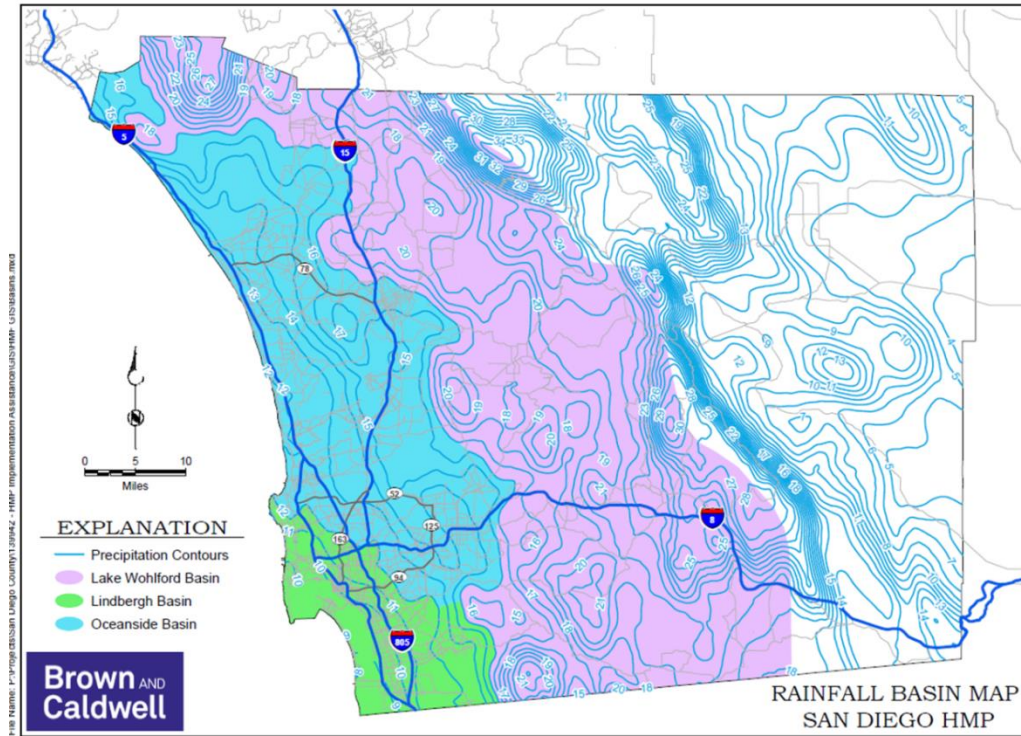
Figure G.2-2.2 Appropriate Rain Gauge for Project Sites
