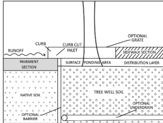
Schematic of Tree Well
