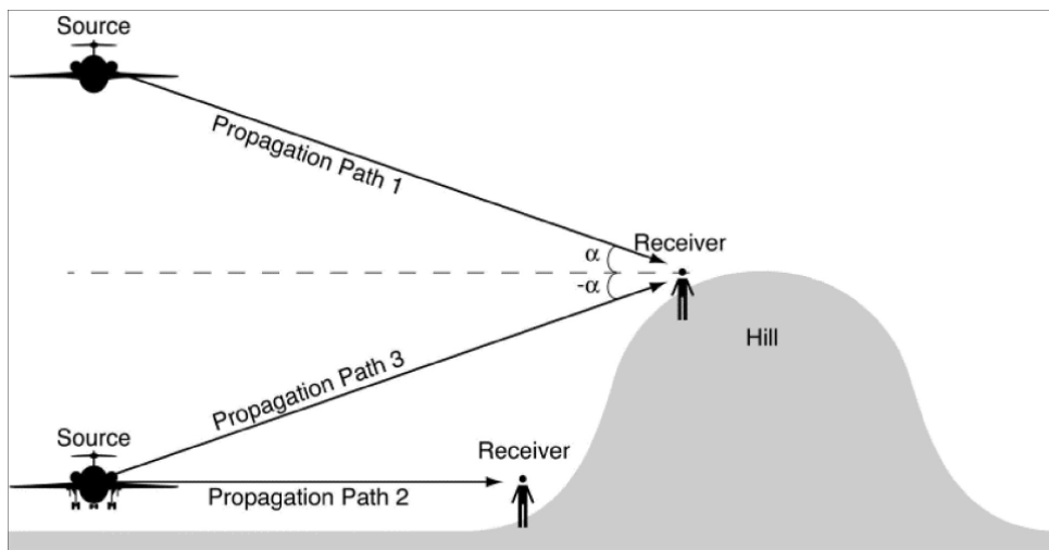
Figure G-2 Aircraft Noise Propagation Paths to Receivers on a Hill Source: HMMH
